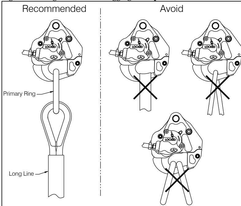
Figure 4.6 Cargo Hook Load Rigging Examples
