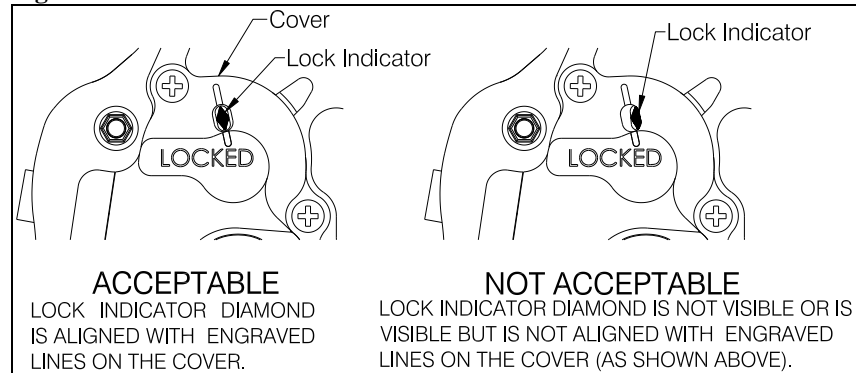
Figure 4.4 Hook Lock Indicator
