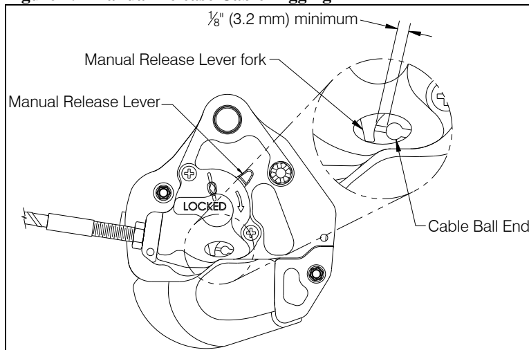
Figure 4.2 Manual Release Cable Rigging
