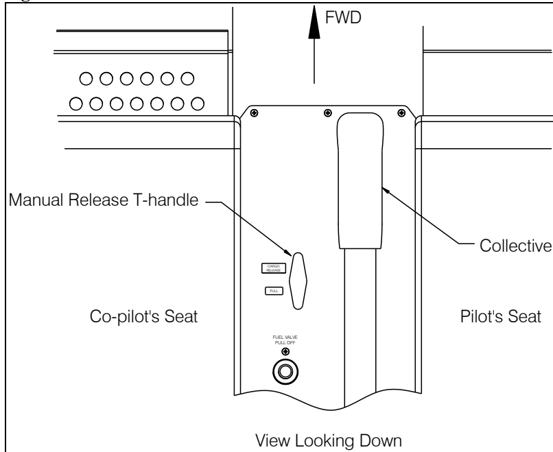
Figure 1.3 T-handle Location
