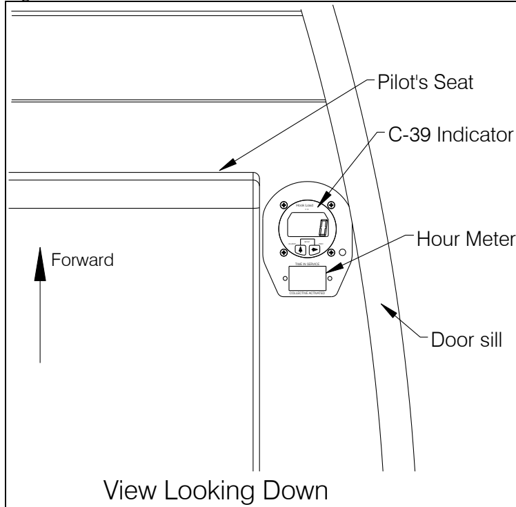
Figure 4.5 C-39 Indicator
